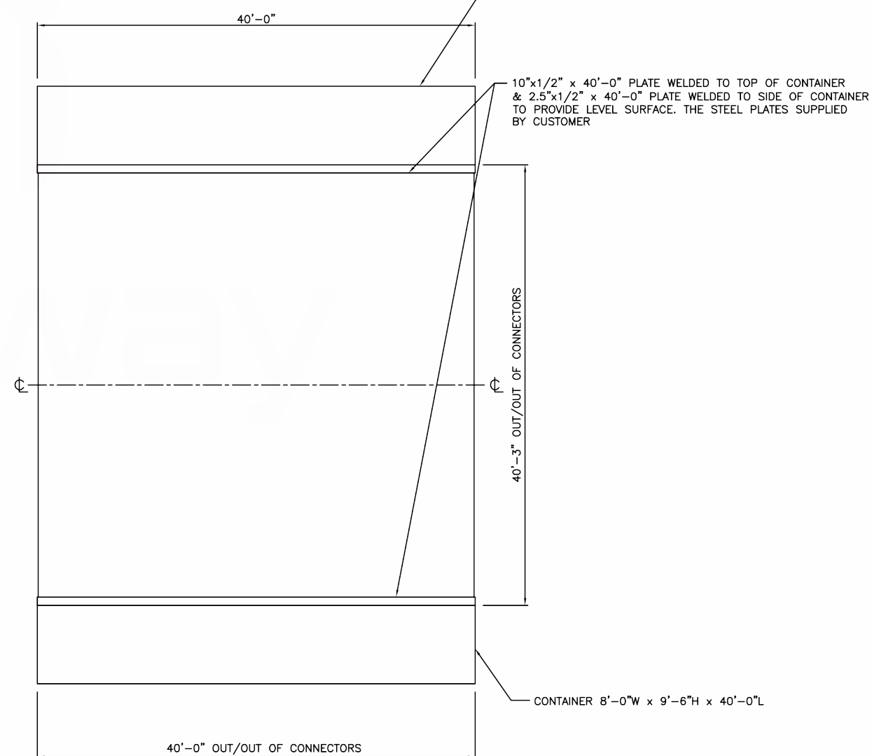
FOUNDATION PLAN
