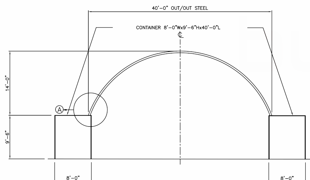
REAR ELEVATION
