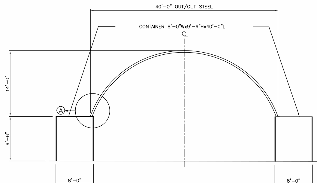
FRONT ELEVATION
