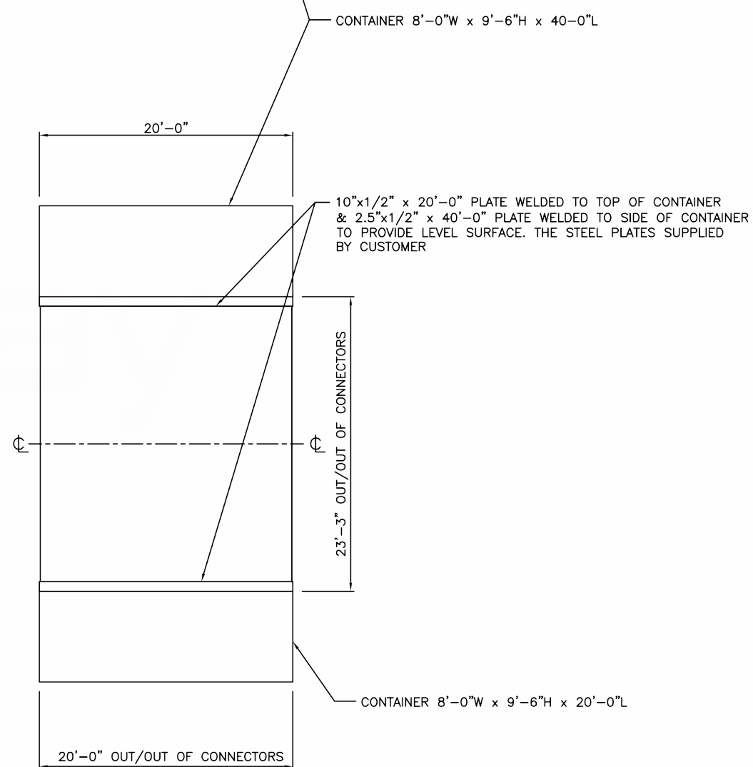
SIDE ELEVATION
