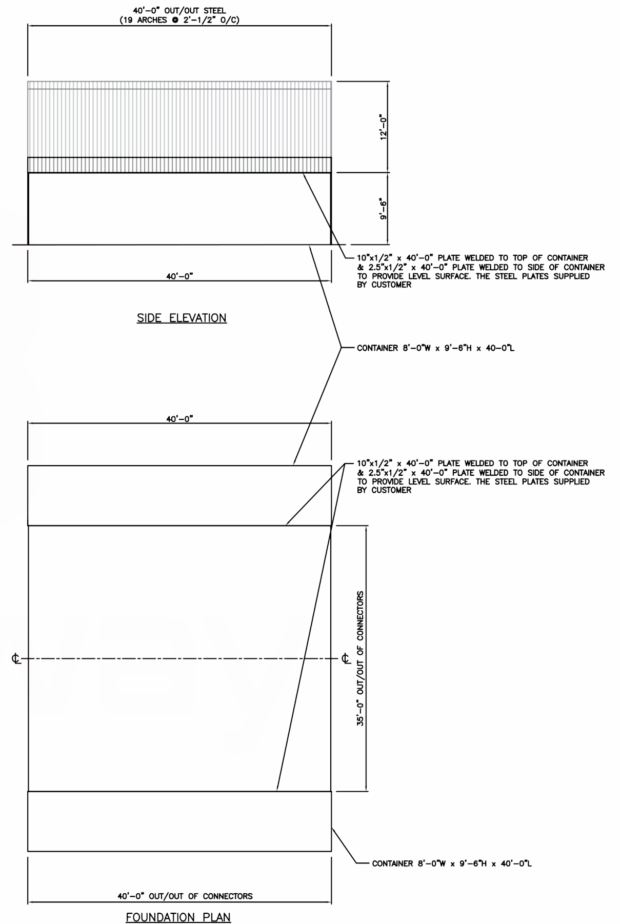
FOUNDATION PLAN
