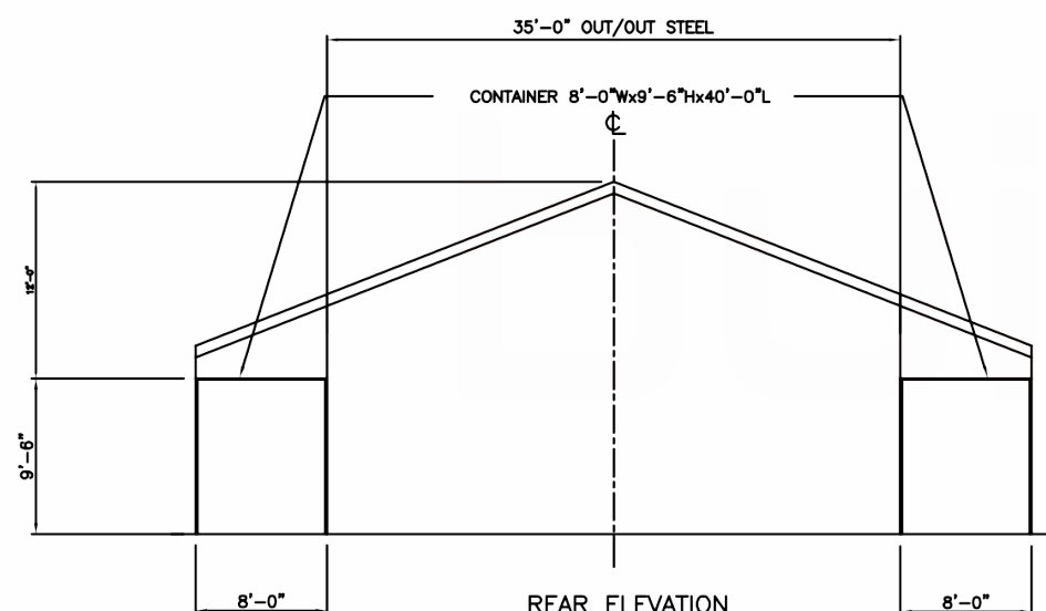
REAR ELEVATION
