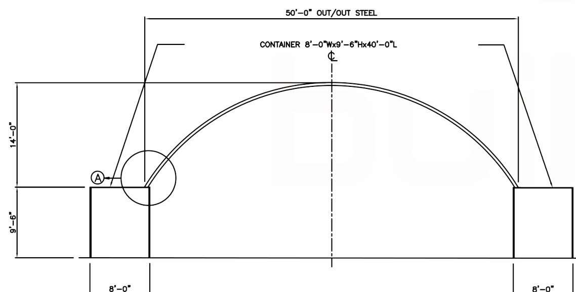
REAR ELEVATION
