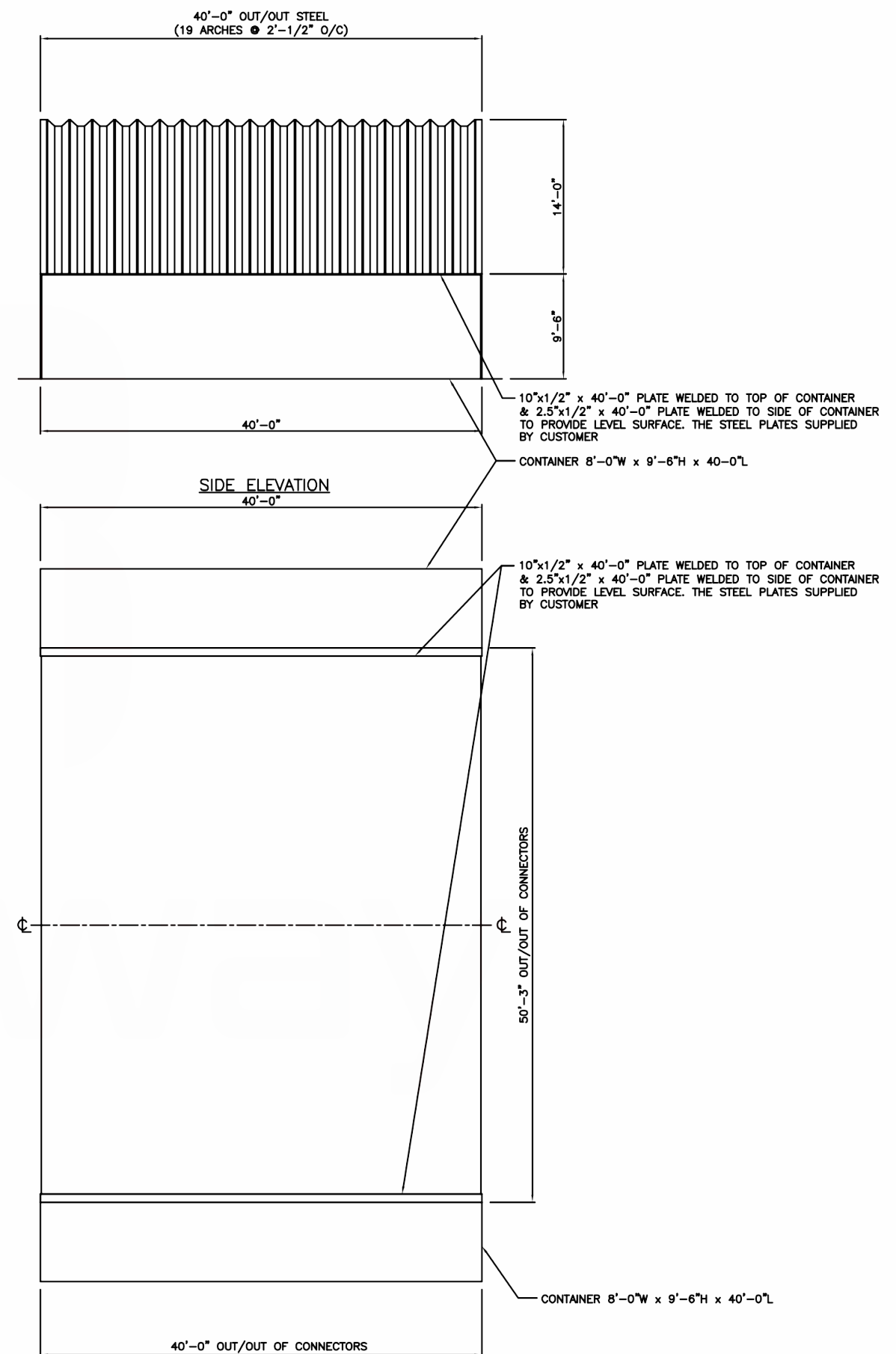
FOUNDATION PLAN
