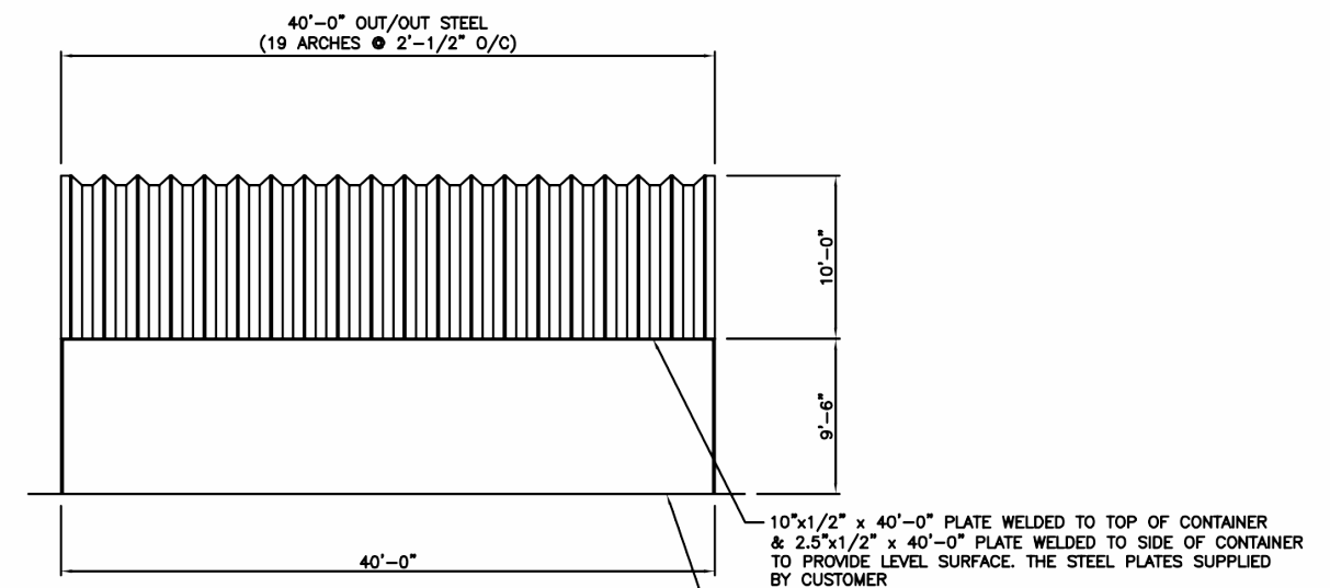
SIDE ELEVATION
