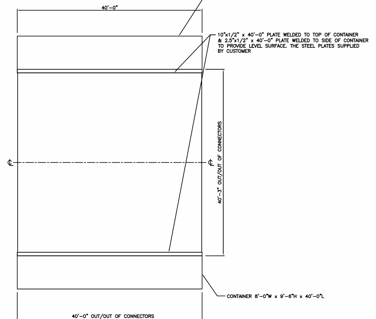
FOUNDATION PLAN
