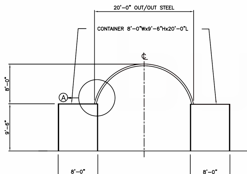
REAR ELEVATION
