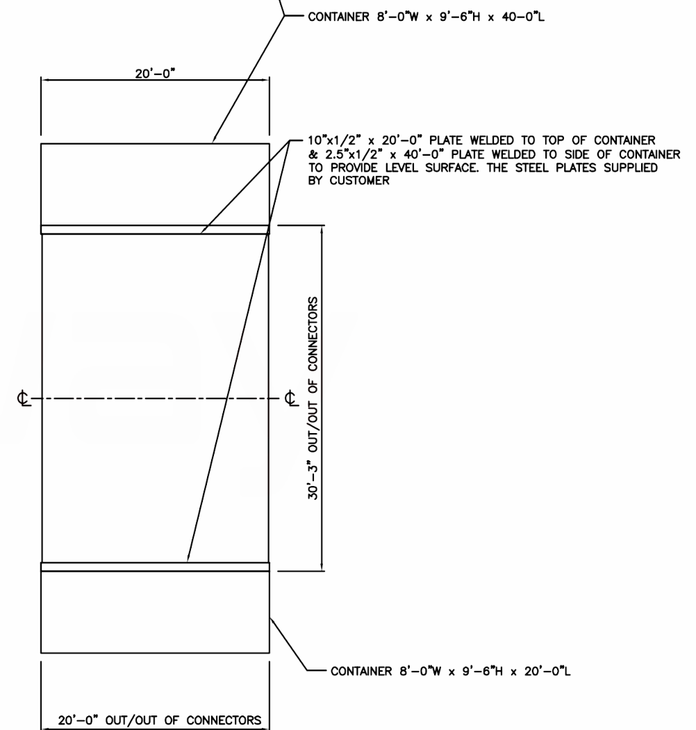
FOUNDATION PLAN
