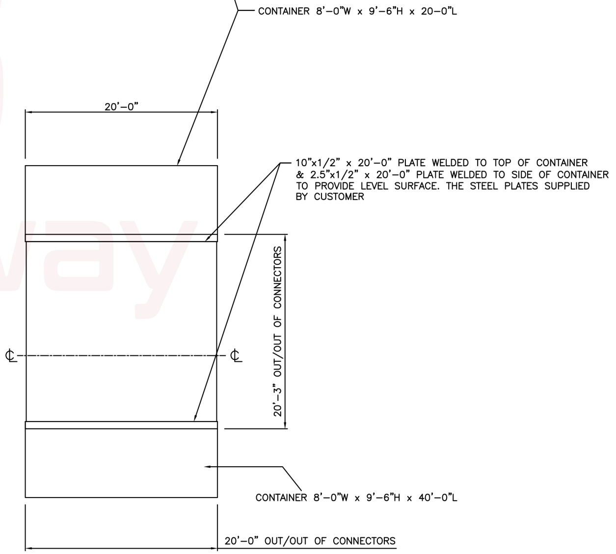
FOUNDATION PLAN
