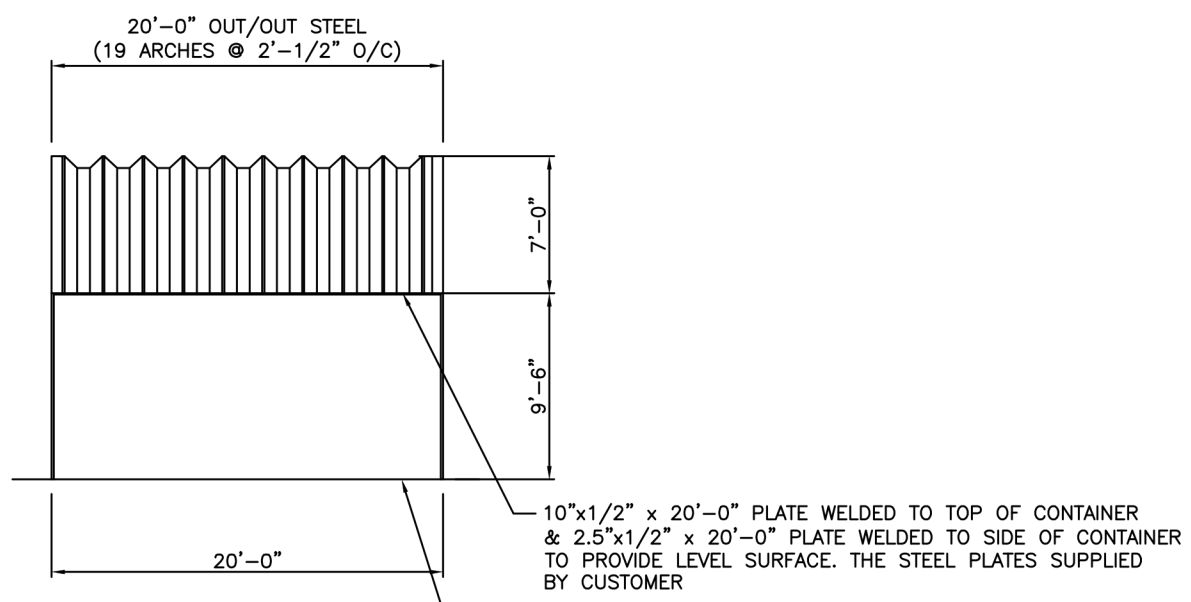
SIDE ELEVATION
