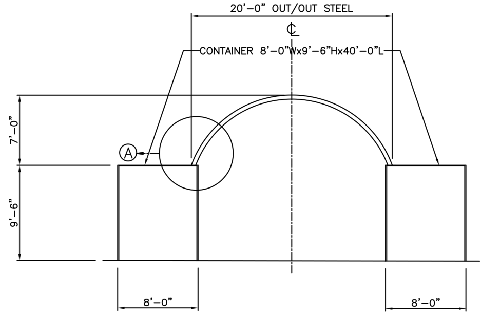
FRONT ELEVATION
